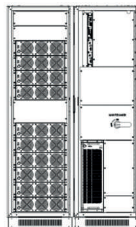
INTERIOR ARMARIO 500kVA
